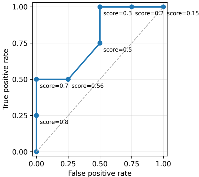
ROC curve, AUC = 0.78125
